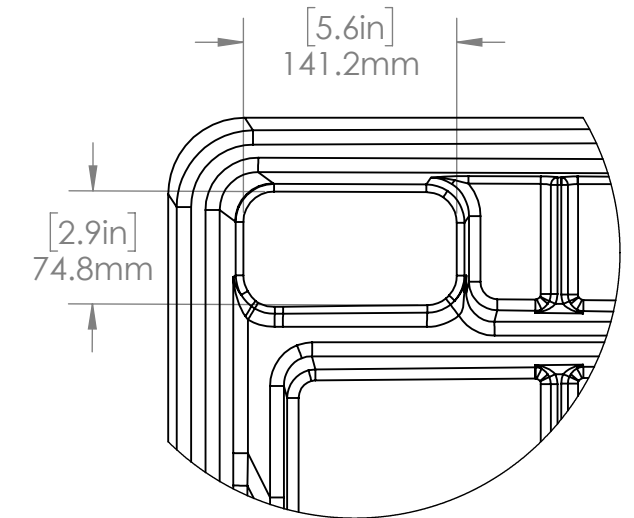
DETAIL B DRAIN AREA
