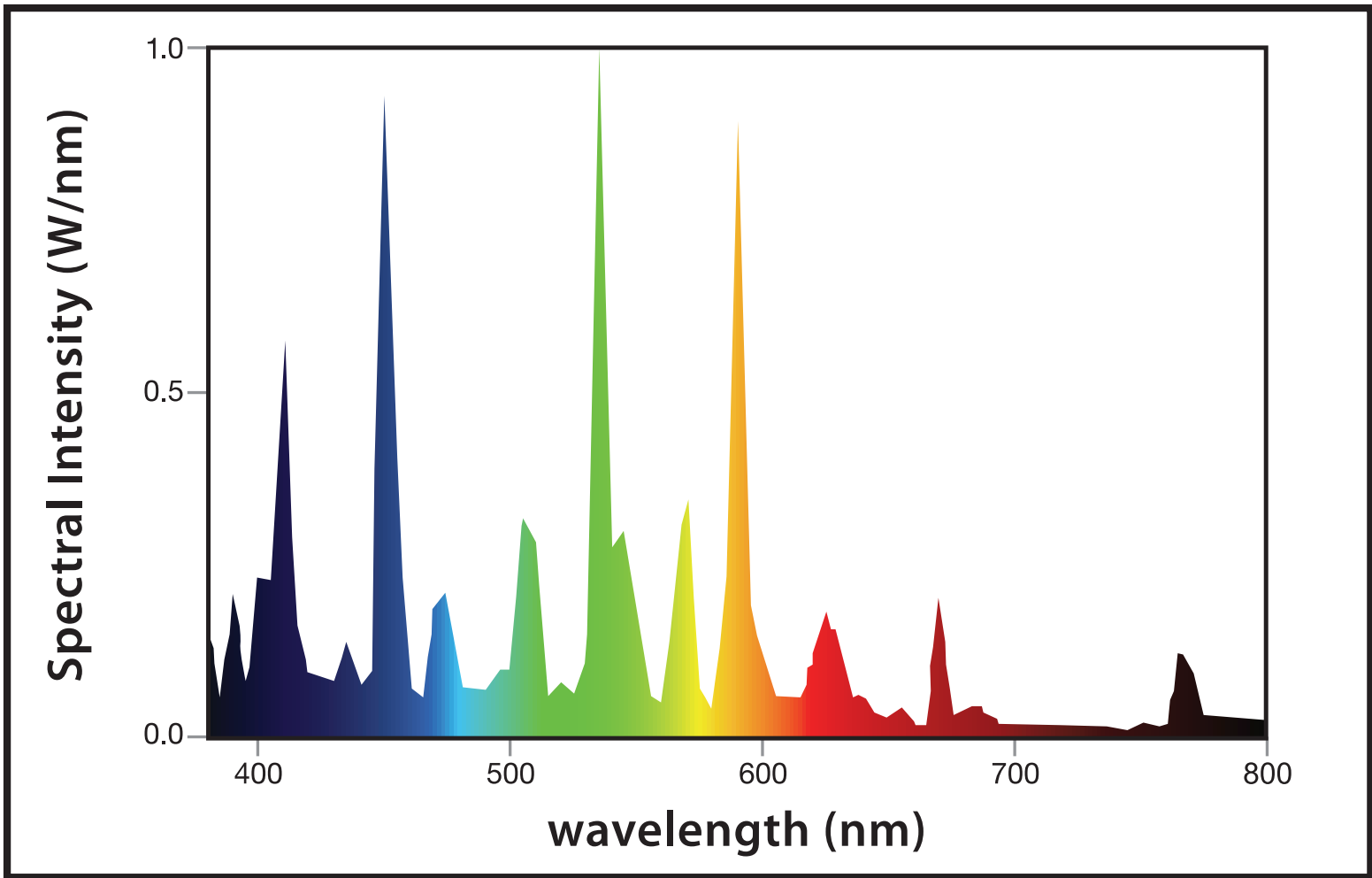
Ultra Sun 1000 Watt - 7,500°K MH Lamp - Spectral Intensity Graph
