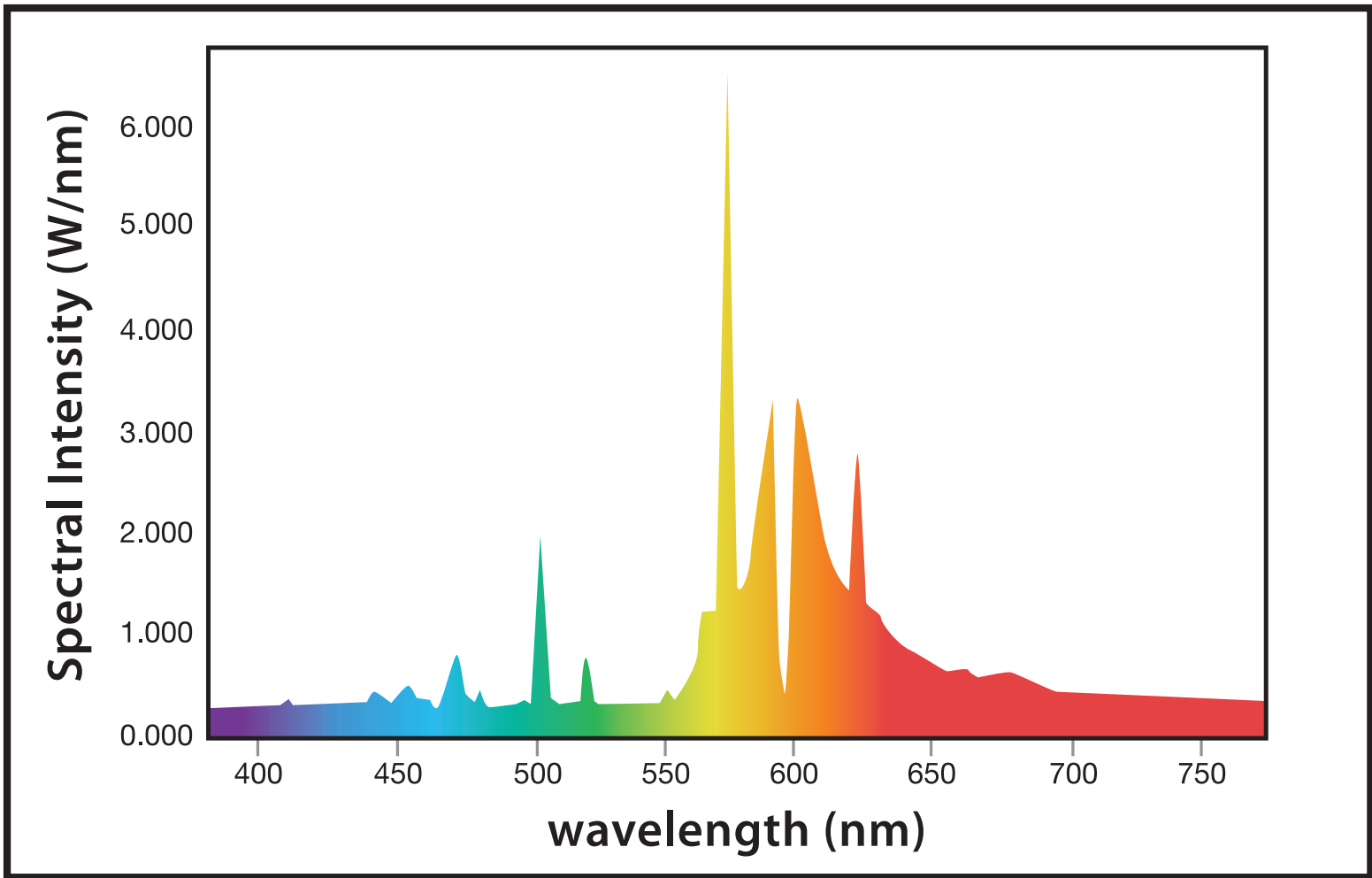
Ultra Sun 600 Watt HPS Lamp - Spectral Intensity Graph
