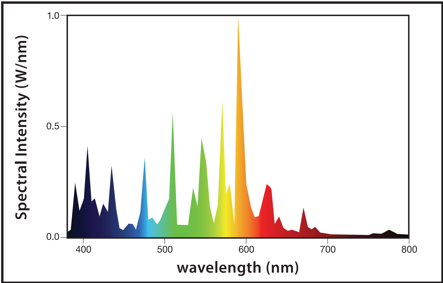
Ultra Sun 1000 Watt - 4,200°K MH Lamp - Spectral Intensity Graph
