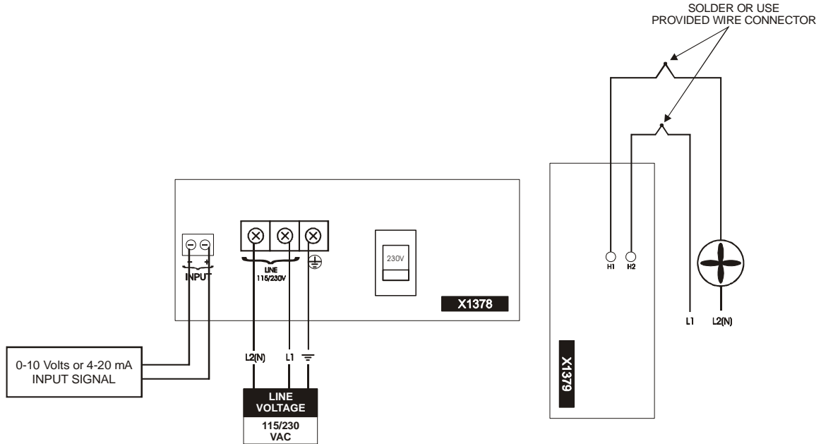
Figure 1: Wiring Diagram
